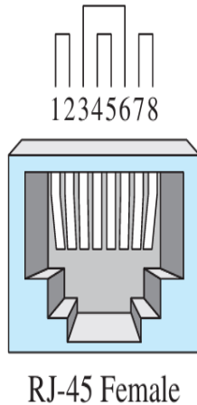
Figure 7.5 UTP connector
